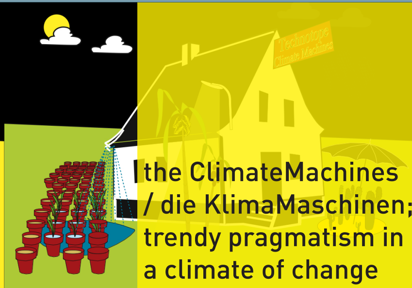
'Climate Machine'
